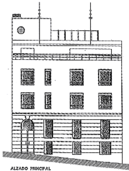
ALZADO PRINCIPAL
